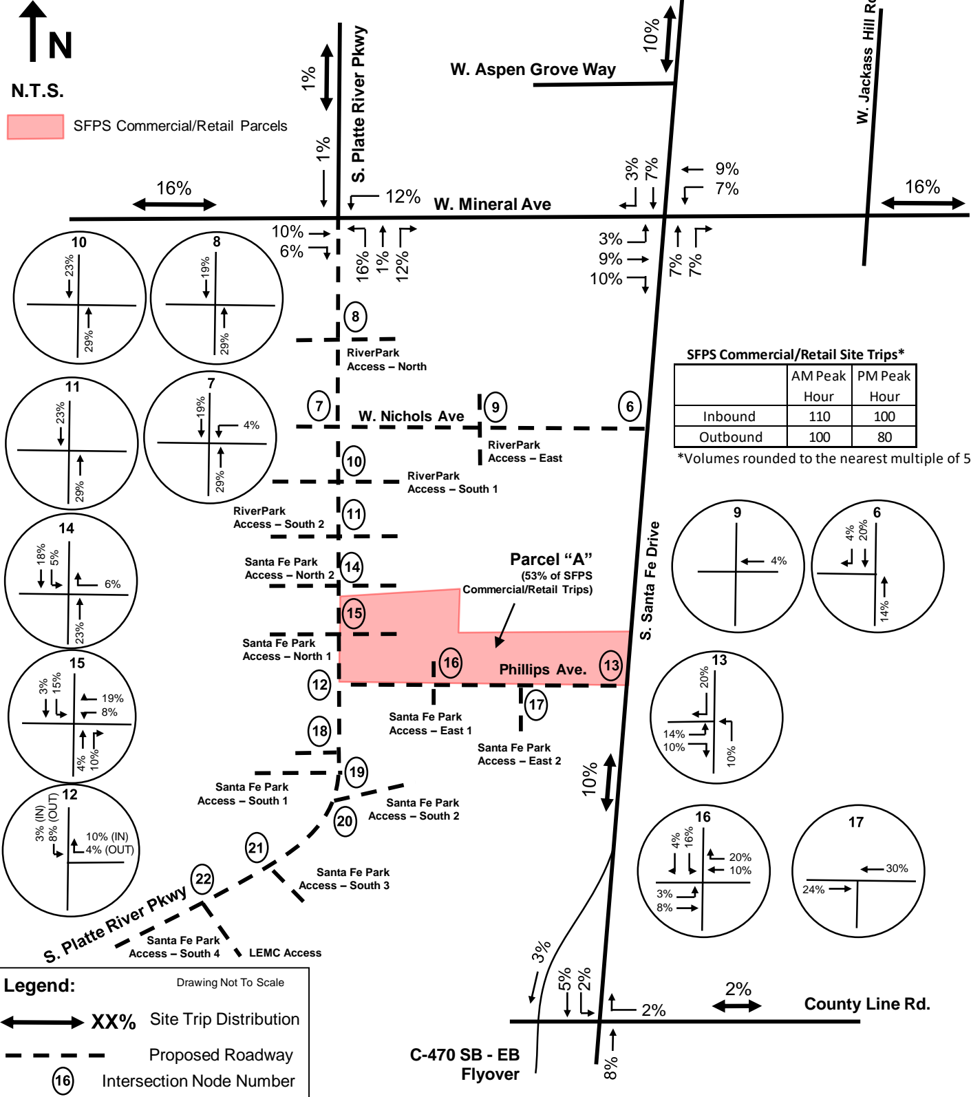
2025 Site Generated Trip Distribution: Santa Fe Park South Commercial/Retail (Parcel "A") Figure 14A
